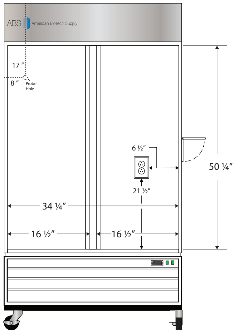
Front View
