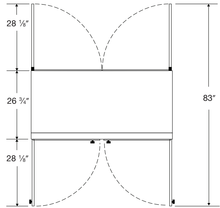
Top View
